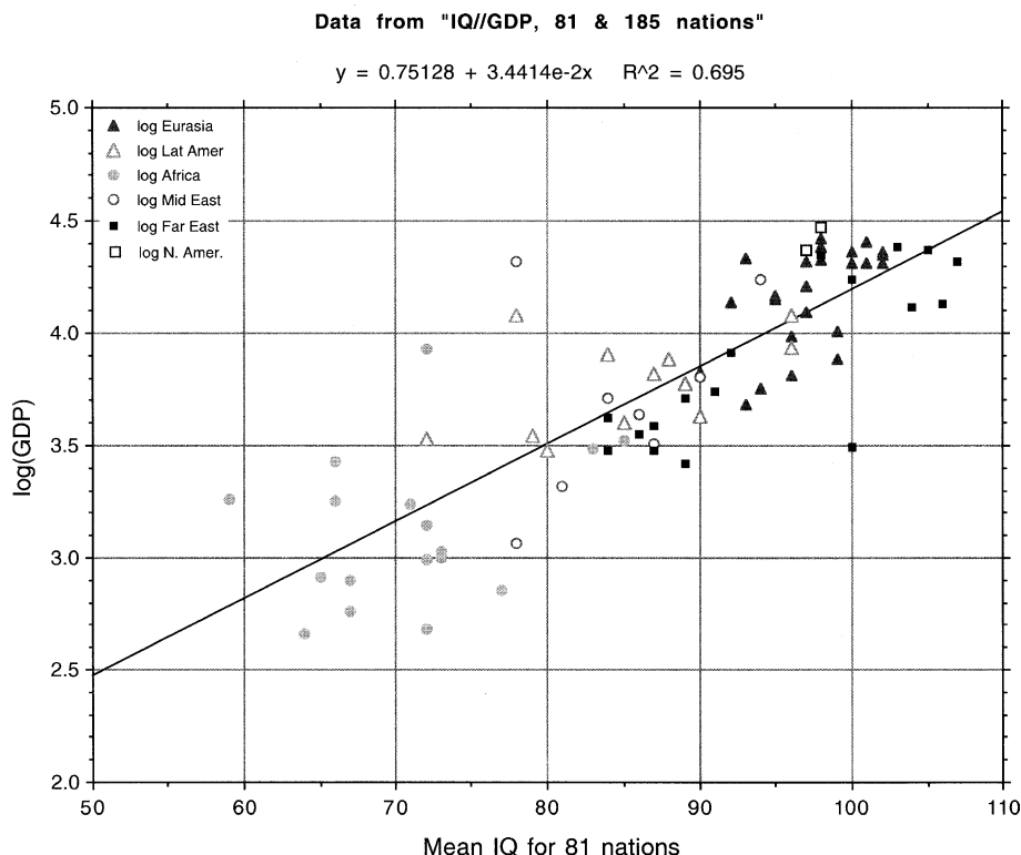
Fig. 3. Conversion of Fig. 1 with exponential fit into a linear plot of \log_{10}(GDP) vs. IQ. The scatter of points is symmetrically distributed in an oval centered around the exponential correlation line. Nations in North America, Eurasia and the Far East cluster at the high end of the line, Mid East and Latin American nations occupy a belt in the middle, and Sub-Saharan African nations appear at lower left. The Lynn/Vanhanen data have been criticized on the grounds that correlations between GDP and IQ are weak below IQ=80 . But it was decided not to alter the full Lynn/Vanhanen data set. As this figure and the following one indicate, deletion of these low-IQ data would not affect the conclusion of linearity of a \log(GDP) vs. IQ plot.
