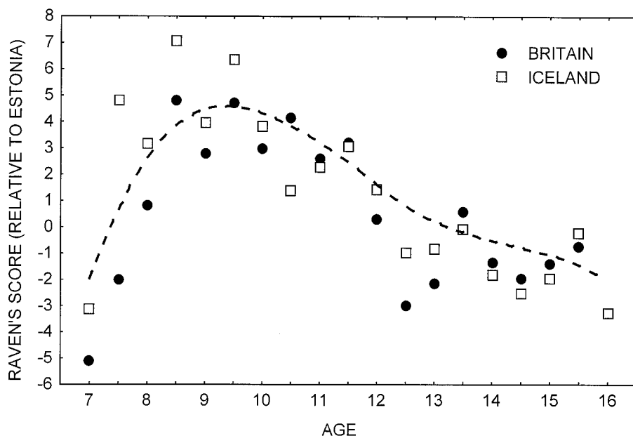
Fig. 1. The Raven's scores of Estonian age groups in relation to British and Icelandic means. British 1979 norms were shifted 3 IQ points up to adjust for the secular increase.
